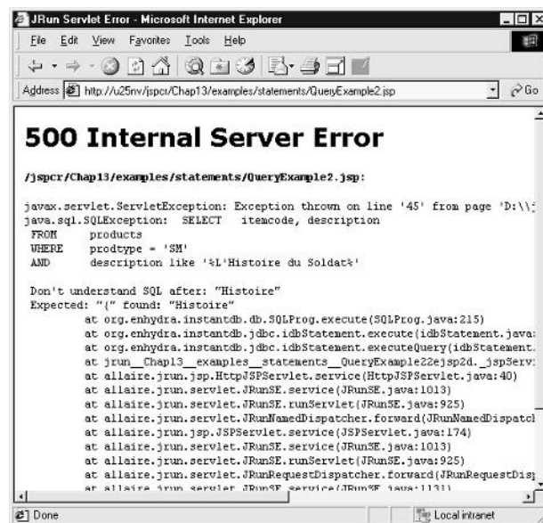
Figure 13-6. Syntax error caused by an unescaped apostrophe
