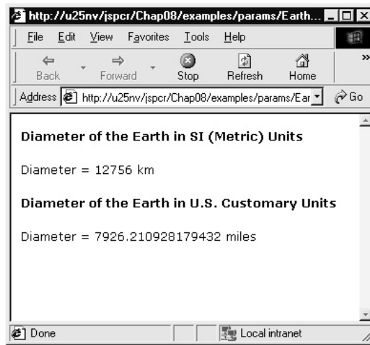
Figure 9-5. A JSP page that includes the same page twice with different parameters
