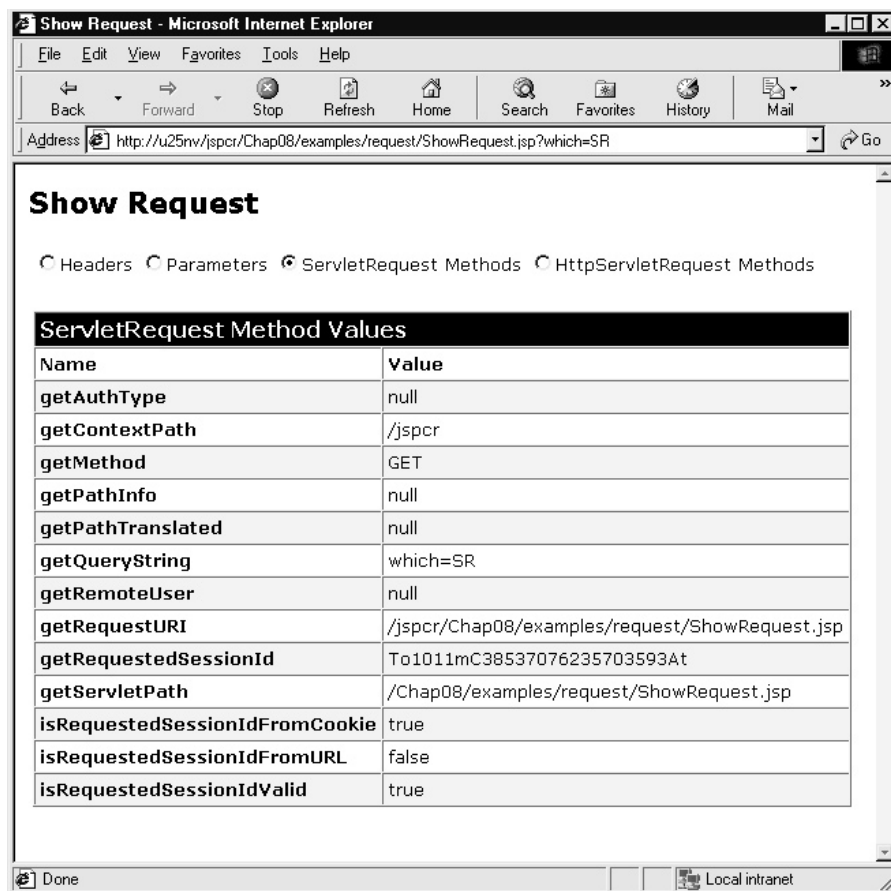
Figure 9-4. Servlet request methods shown in the third tab of ShowRequest.jsp
