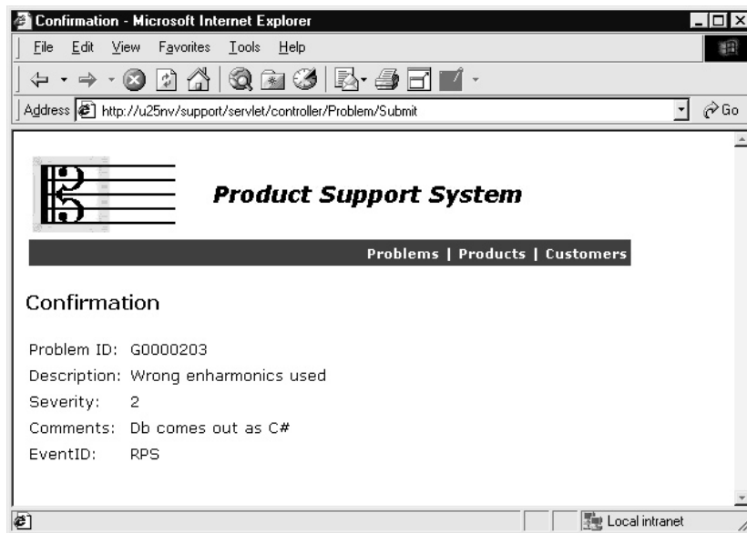
Figure 19-8. Confirmation page
