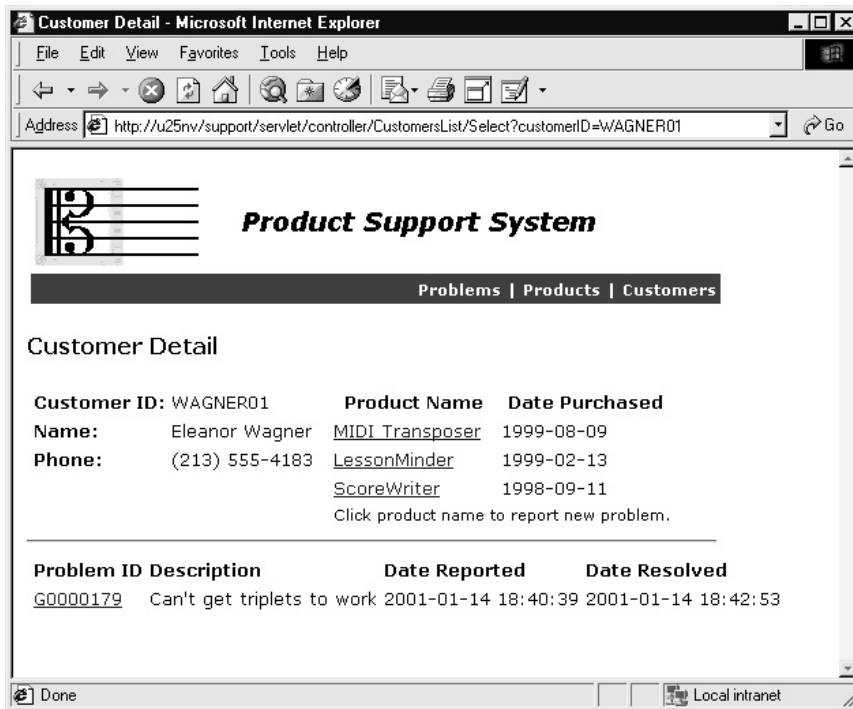
Figure 19-6. Customer detail page
