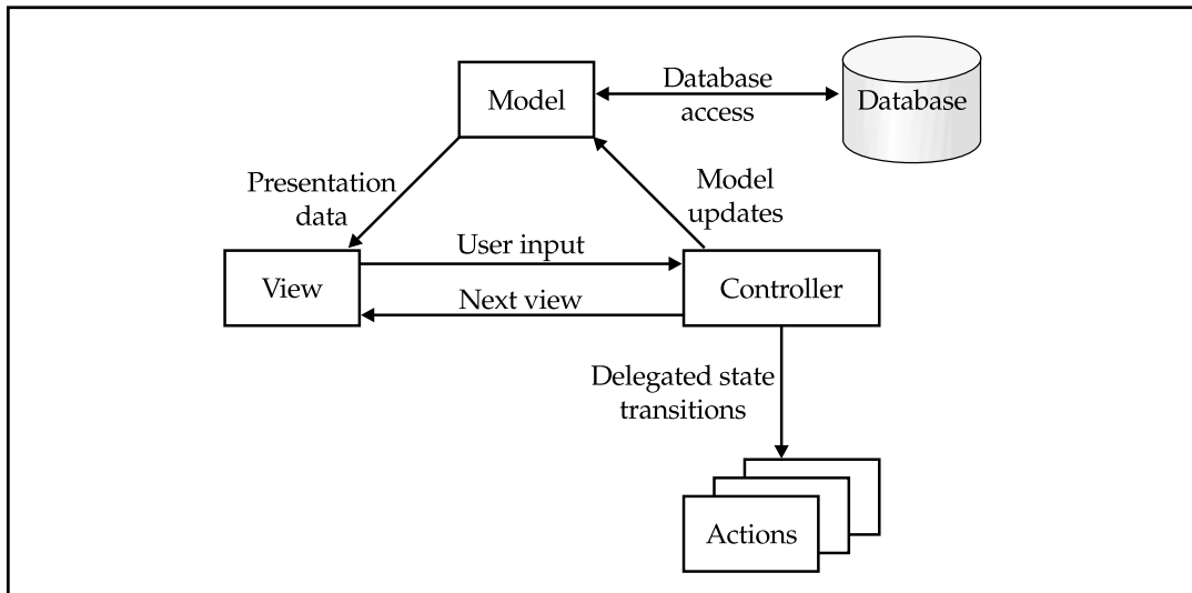
Figure 19-2. The Model-View-Controller architecture
