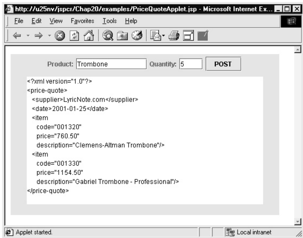
Figure 20-1. Results of running PriceQuoteApplet
