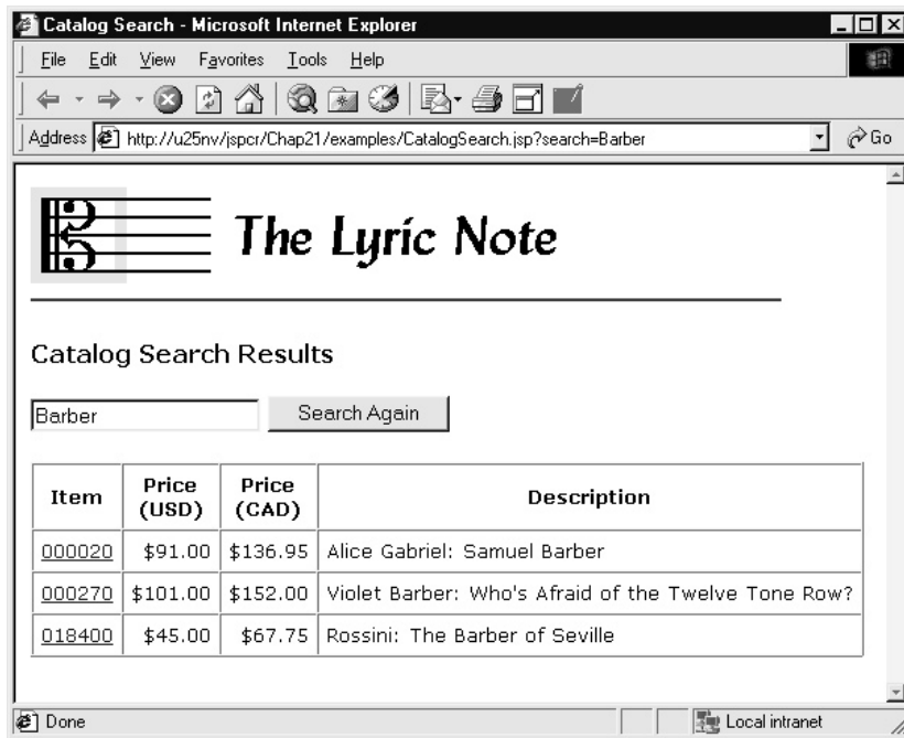
Figure 21-1. Catalog search output illustrating USD-CAD exchange rates obtained from CGI resource
